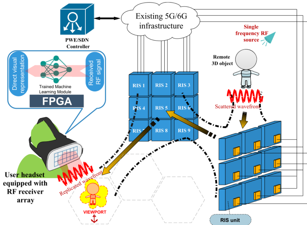
FIGURE 2. The iCOPYWAVES end-to-end system workflow, overviewing the steps from the creation of an RF scattered wavefront from a remote object, to its visual representation at the user's headset.
