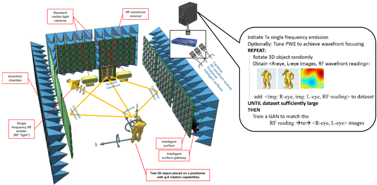
FIGURE 3. Overview of the envisioned iCOPYWAVES GAN training phase (which occurs offline), showcasing the successful translation of RF readings into visual representations of the corresponding 3D objects.
