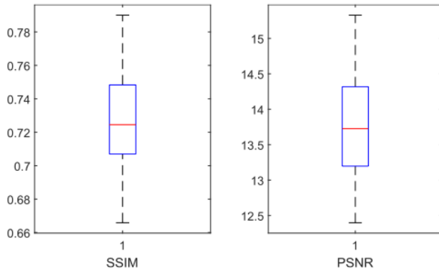
FIGURE 8. Boxplots of the attained SSIM and PSNR image comparison values over 100 object reconstructions via iCOPYWAVES.
