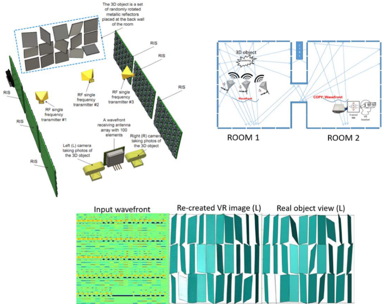
FIGURE 7. Validation setup: an XR-RF imaging process in a simple room (top left), where the 3D object is a set of randomly rotated rectangular reflectors placed on a wall. Three RF transmitters (yellow horn antennas) emit 5 GHz waves upon the 3D object which scatter around it, and an antenna array with 100 elements gets a corresponding reading. Two standard cameras—(L)eft and (R)ight—take visual snapshots of the 3D object. The process is repeated 1000 times, each time rotating the 3D object randomly, thus, creating a dataset for training a GAN [83], which then translates an RF reading to a visual outcome. Once the training is complete, a second room is added to the layout with all walls covered with metasurfaces (top right). The original wavefront is copied from room 1 to another place in room 2. The trained GAN recreates the visual snapshot (bottom).
