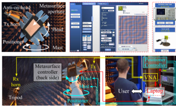
FIGURE 11. The contributed testbed for realizing an XR copying wavefronts/wavevolumes system. Clockwise, from top left: Close-up photo of a metasurface loaded on an automated positioner and illuminated by a fixed source; screenshots from the developed software that calculates and assigns configurations to a metasurface, and directs the measurement setup.
