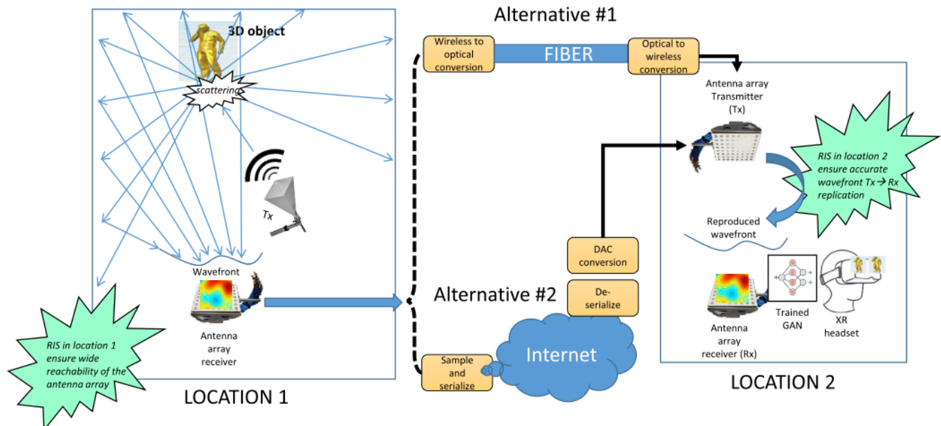
FIGURE 5. Overview of the first approach for remote operation. This scenario requires a receiving antenna array in location 1, and a transmitting antenna array in the remote location 2. The goal is to transfer the wavefront impinging over the receiving antenna array in location 1 over direct fiber (wireless-to-optical happens at the physical layer with practically zero latency). In lack of fiber availability, the Internet can be used as a common alternative. Within location 2, the PWE handles the wavefront replication from the Tx to the Rx (collocated with the user's XR headset). This approach requires regular SDMs, without wavefront sensing capabilities. Additionally, we note that this approach is also the default way for carrying all complementary information, such as sound and any sensor (e.g. haptic) feedback.
