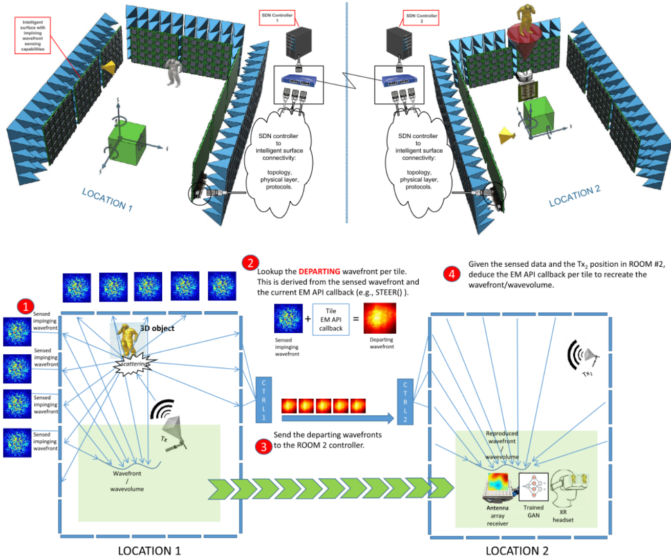
FIGURE 6. Overview of the second approach for remote operation. (Top) Showcasing the copying of a wavefront carrying XR visualization in an indoors environment. This approach does not require extra antenna arrays, while it is able to replicate wavevolumes as well as wavefronts. (Bottom) Workflow for the “over-the-wire” reproduction of the intended wavefront/wavevolume. This approach requires advanced SDMs, with wavefront sensing capabilities.
