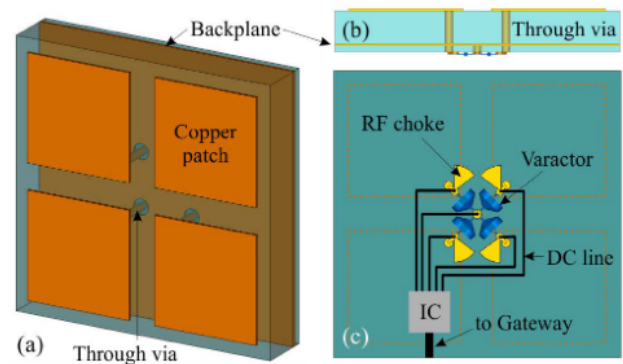
FIGURE 12. (a) Perspective top-side view of a unit cell composed of a 2 \times 2 array of square patches; this cell topology allows independent control of reflection amplitude and phase in both polarizations. (b) Side view of the unit cell, showing the through vias connecting the patches at the top side to the actuators embedded in the bottom side. (c) Bottom side view of the unit cell, where the actuators here correspond to varactors, i.e., DC-voltage controlled variable capacitors; an IC embedded in the cell receives commands from the gateway and applies voltages to each of the four varactors effectively setting the cell response; note that microwave engineering is required here, e.g., RF chokes to isolate the DC/RF lines.
