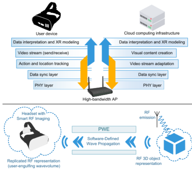
FIGURE 1. High-level comparison between the existing full-stack solutions for XR (top) and the proposed iCOPYWAVES approach (bottom), whose operation remains bounded within the physical layer.
