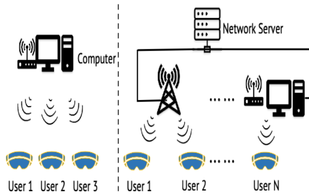
Fig. 6 – Multi-user LAXR (left) and WAXR (right) systems.
