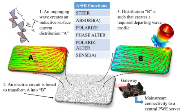
Fig. 1. Operating principle of intelligent surfaces based on the generalized internetworked metasurface concept (HyperSurface).
