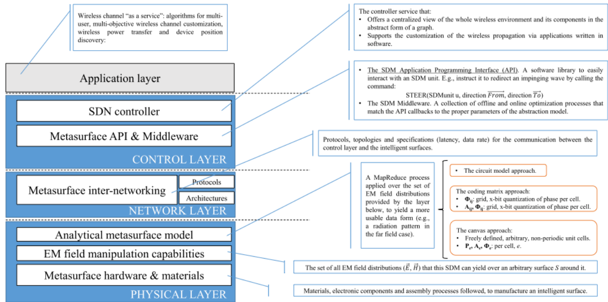
Fig. 4. Functionality layer approach for organizing the ongoing research efforts in the literature.
