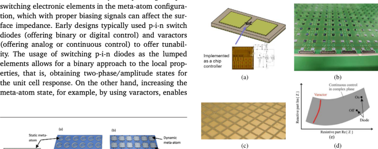
Fig. 6. Metasurface example: (a) example realization of controller chip, (b) fabrication of controller chips on back plane of metasurface, (c) fabrication of front plane of metasurface, and (d) operating range of tunable lumped elements: diode, varactor, and tunable controller chip.
