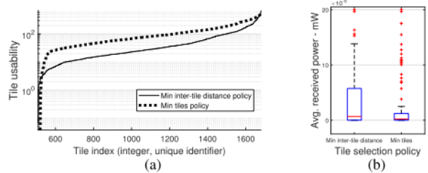
Fig. 12. Deployment statistics for the selection policies of Fig. 11. (a) Distribution of the tile usability per policy. (b) Received power distribution per policy.
