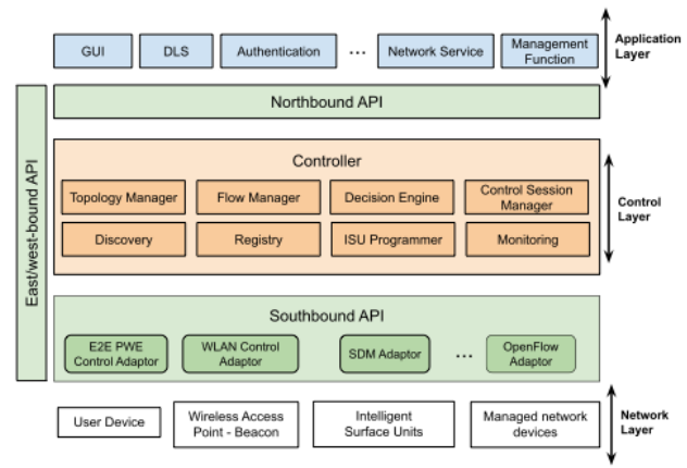
Fig. 7. PWE/SDN controller architecture.
