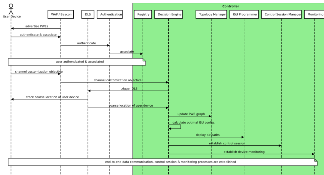
Fig. 8. Message exchange diagram of exemplary end-to-end PWE system workflow.
