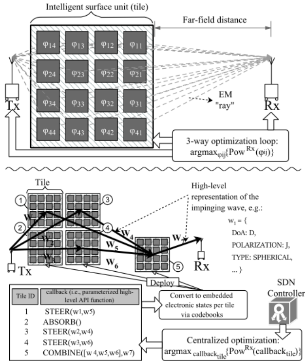
Fig. 3. Different PWE optimization approaches in the literature. Top: SREs favor the flat optimization approach. Bottom: PWEs favor the hierarchical approach targeting multisurface deployments and real-time operation.
