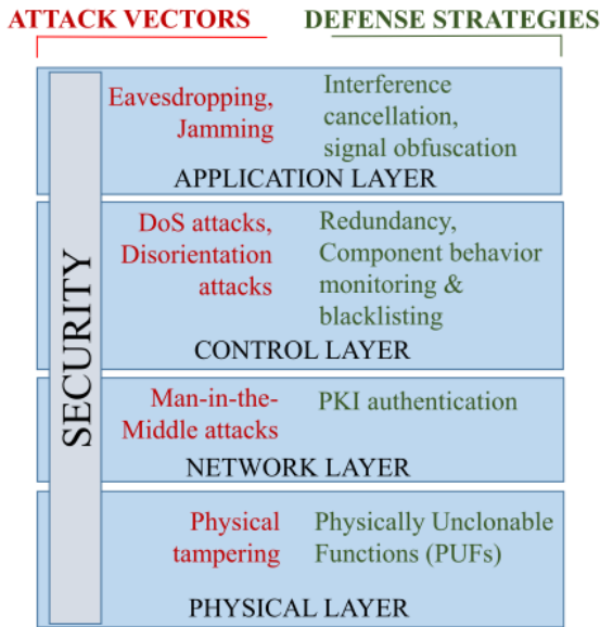
Fig. 13. Security challenges for intelligent environments per system layer.
