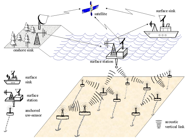
Figure 2: 3D Underwater Sensor Networks
