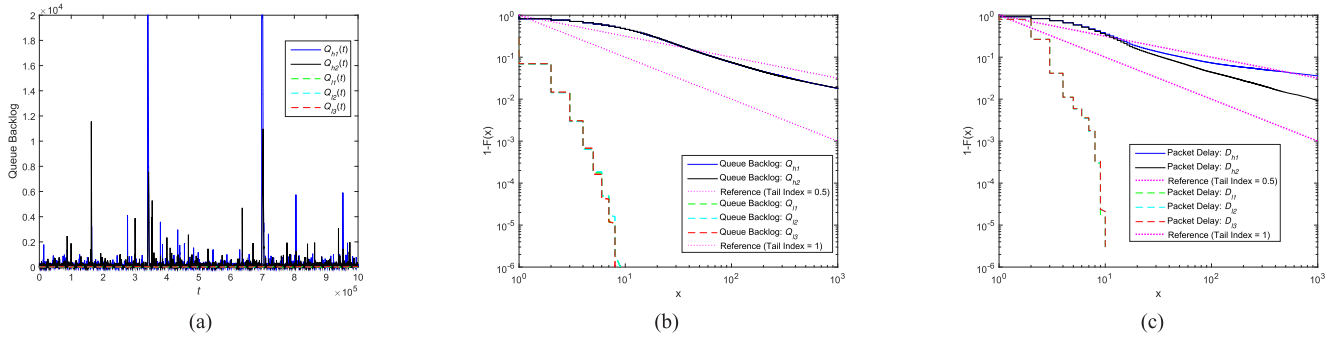
Fig. 3. Queue lengths and packet delay under the DMPWS policy, where network is stable. (a) Evolution of queue lengths. (b) Tail distribution of queue lengths. (c) Tail distribution of packet delay.
