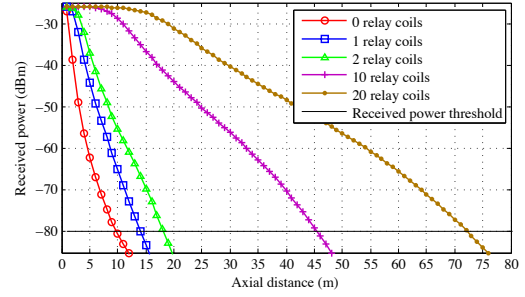
Fig. 2. Received power of MI waveguides with different relay coil numbers.
