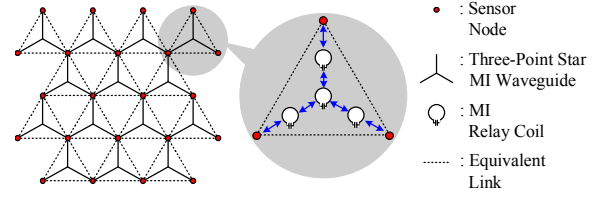
Fig. 3. The MI waveguide deployment using TC algorithm in the WUSN with hexagonal tessellation topology.
