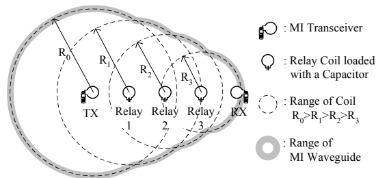
Fig. 1. The structure and the communication range of a MI waveguide.
