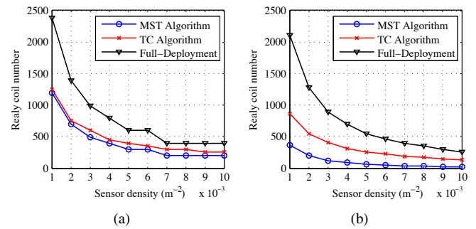
Fig. 5. The number of relay coils to connect 100 sensors in WUSNs with (a) hexagonal tessellation topology and (b) random topology.
