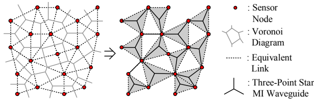
Fig. 4. The MI waveguide deployment using TC algorithm in the WUSN with random topology.
