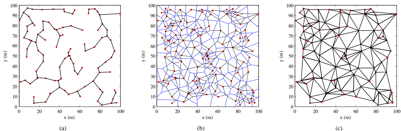
Fig. 6. The deployment results of (a) the MST algorithm, (b) the TC algorithm, and (c) the full-deployment strategy. (The red dots are the sensors; the black lines are the MI waveguides; and the blue cells are the Voronoi diagrams. 100 sensors are uniformly distributed with a spatial intensity \lambda_{rand} = 0.01 \text{ m}^{-2} .)
