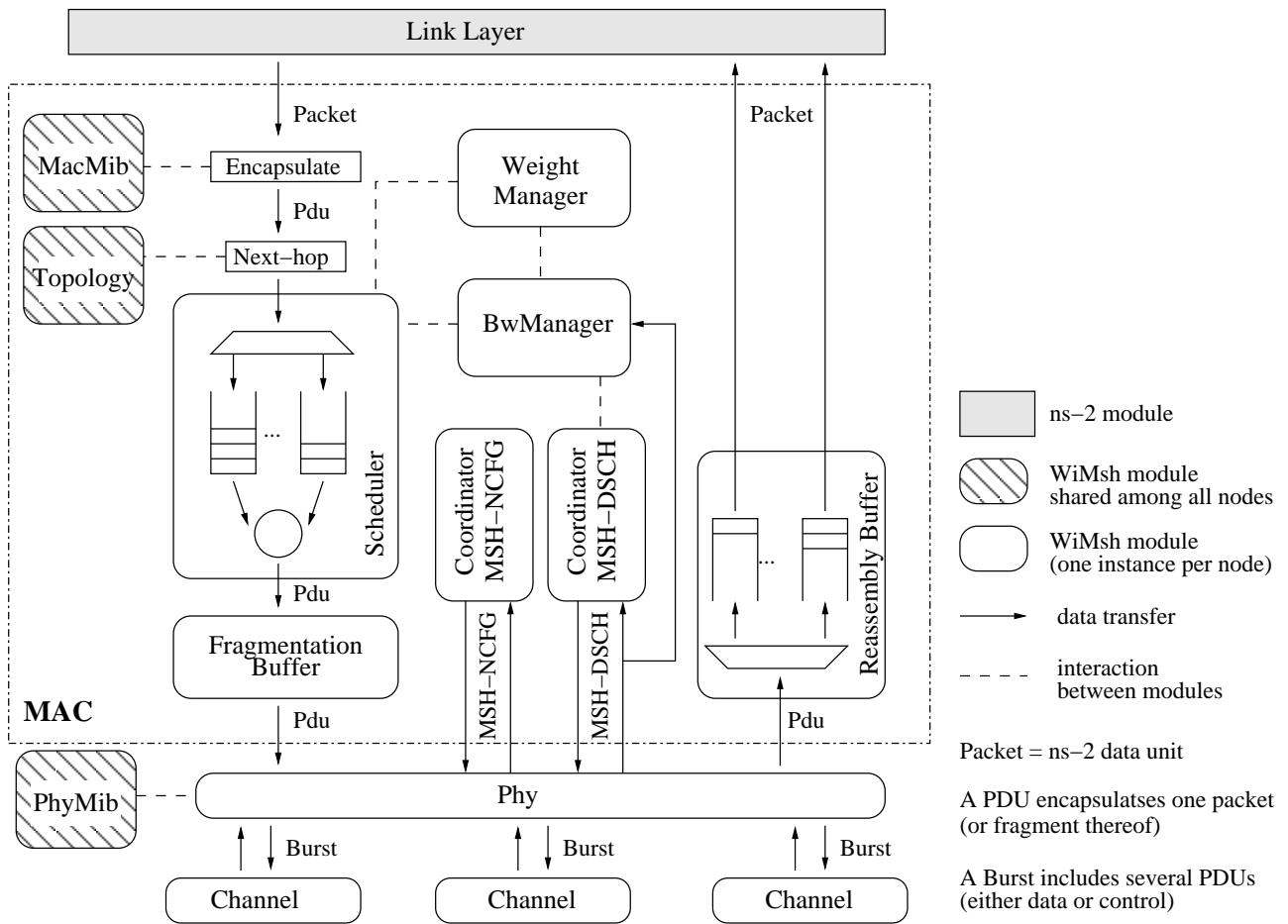
Figure 2: The WiMSh architecture.
