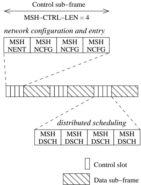
Figure 1: Example of frame structure.
